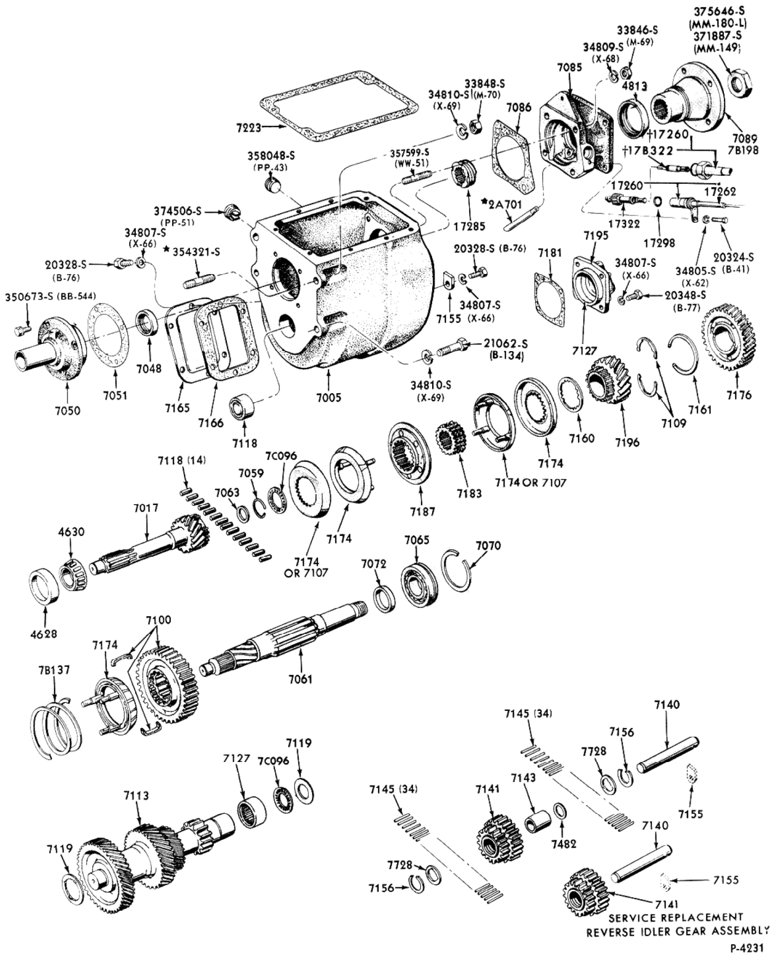
TRANSMISSION - 4 SPEED SYNCHRO. HELICAL GEAR (NEW PROCESS 435) 1964/72 B-C-F-N100/700
